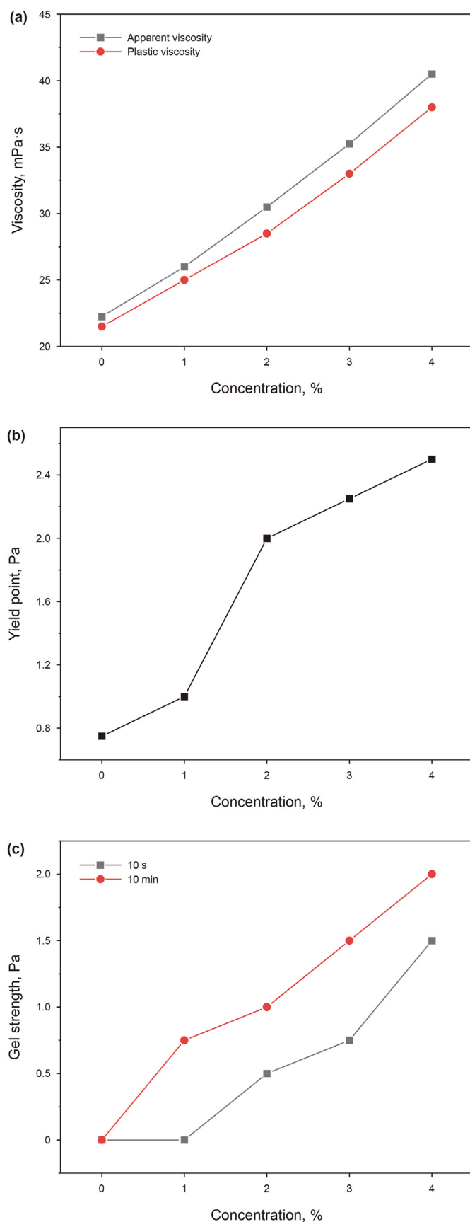
Fig. 7. Variation of rheological parameters for drilling fluid with HSR concentration at -55 °C ((a) viscosity; (b) yield point; (c) gel strength).
