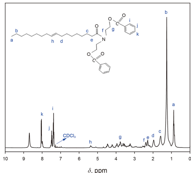
Fig. 3. ^1\text{H} NMR diagram of HSR.
