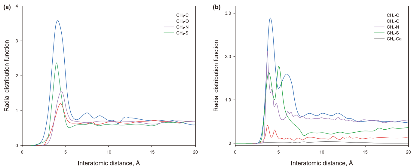
Fig. 14. Radial distribution function between methane and atoms in the system under the same temperature and pressure conditions: (a) kerogen system; (b) calcite kerogen composite model system.
