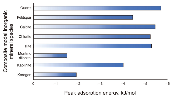
Fig. 13. Peak adsorption energy of different composite models under the same temperature and pressure conditions.
