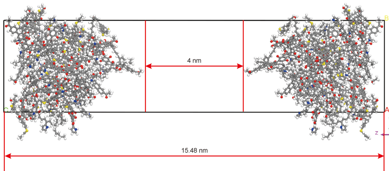
Fig. 3. 4 nm slit pore model of two layers of kerogen organic matter.
