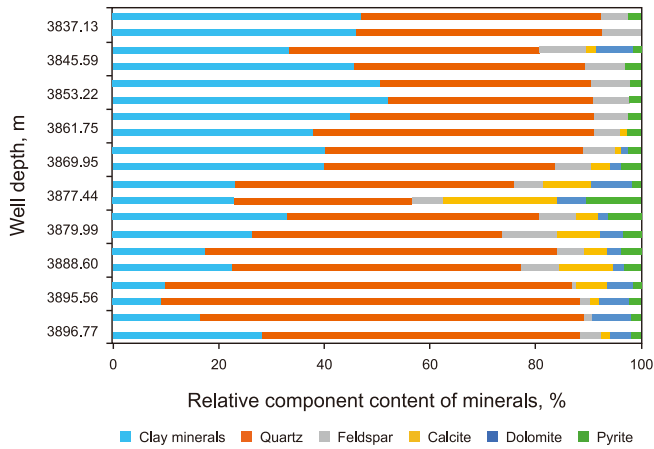
Fig. 5. Relative composition of shale minerals in the Longmaxi Formation of the Sichuan Basin.
