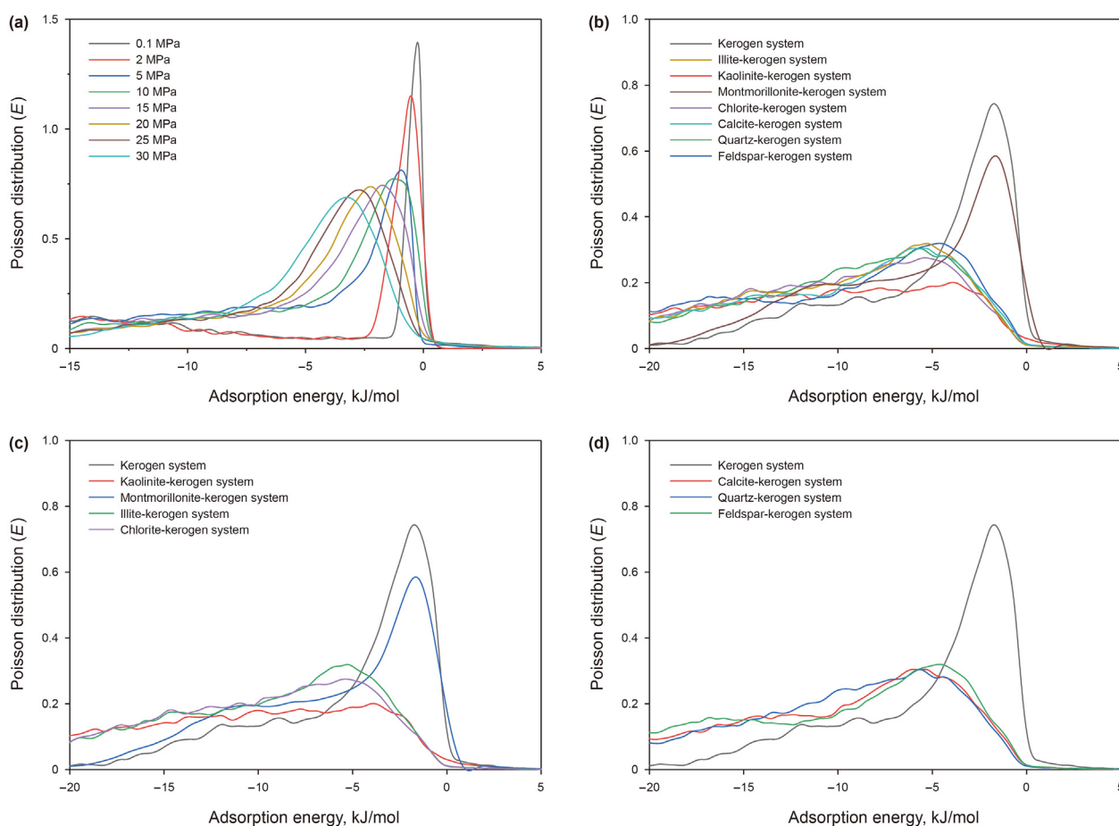
Fig. 12. Adsorption energy distribution curves of methane by different systems at the same temperature. (a) Kerogen system; (b) composite model systems of different minerals; (c) clay-mineral composite model system; (d) non-clay mineral composite model system.
