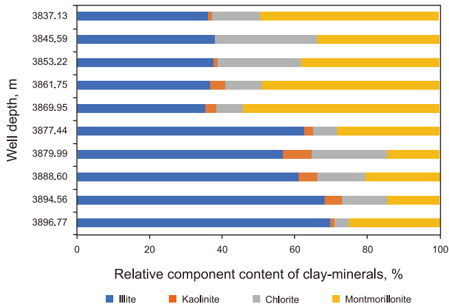
Fig. 6. Relative composition of clay minerals in the Longmaxi Formation shale of the Sichuan Basin.
