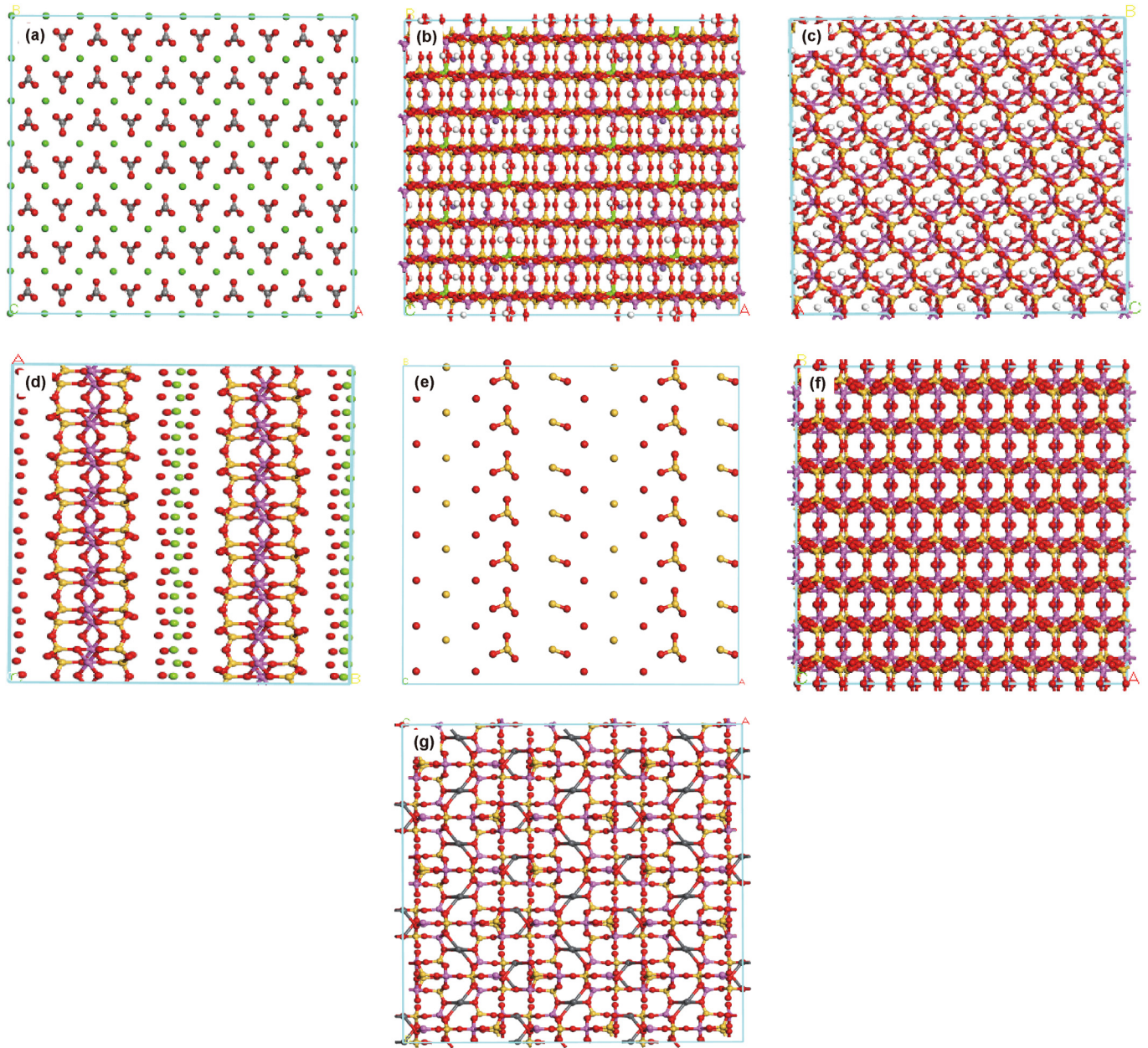
Fig. 7. Presents the three-dimensional structures of the inorganic mineral models. (a) Calcite, (b) montmorillonite, (c) kaolinite, (d) chlorite, (e) quartz, (f) illite, (g) feldspar.
