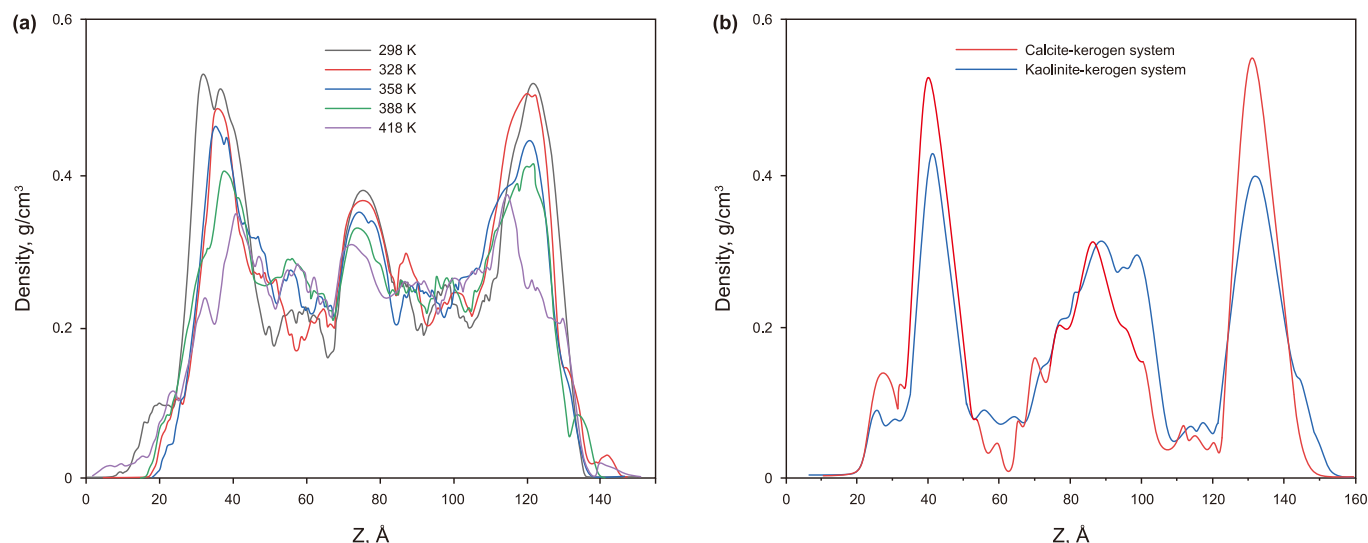
Fig. 15. Density distribution curves in the slits of different methane systems at a constant pressure: (a) kerogen system; (b) composite model systems of different minerals.
