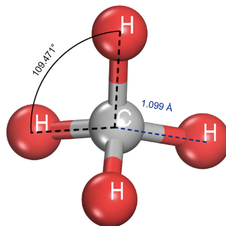
Fig. 4. Optimized methane molecular model.
