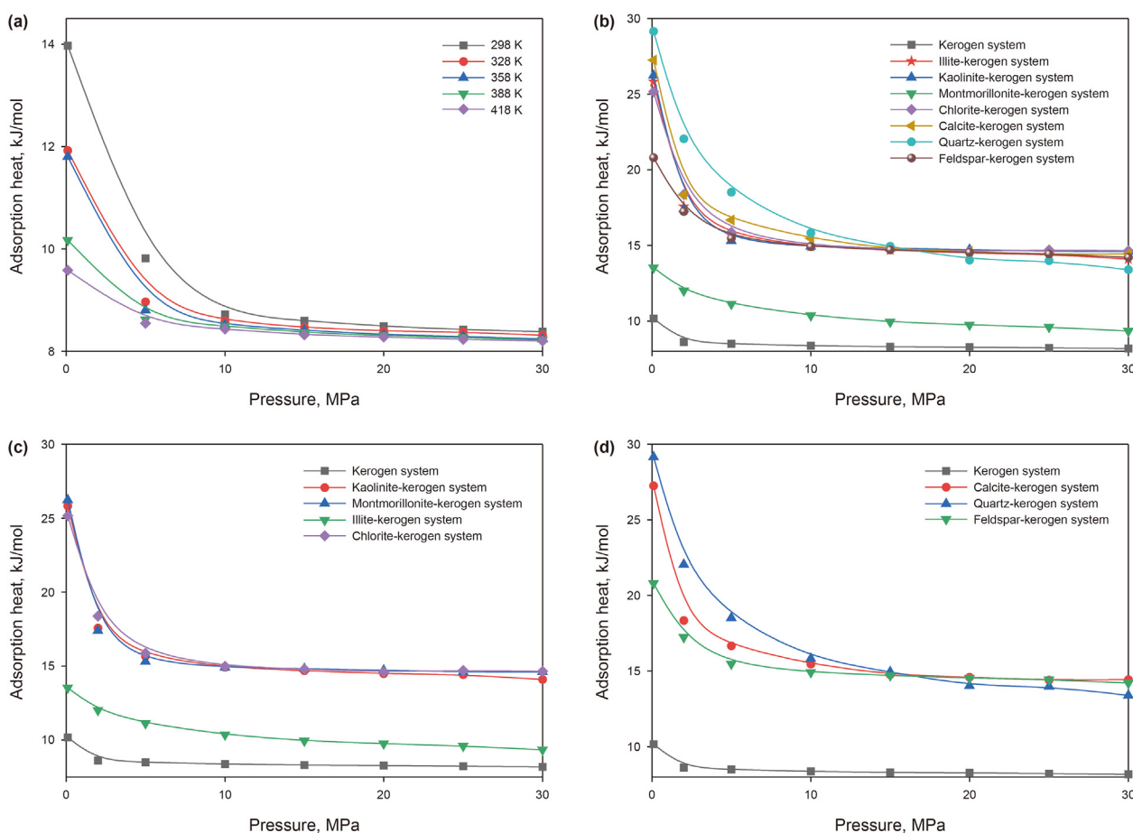
Fig. 11. Average isometric adsorption heat curves of methane under different systems. (a) Kerogen system; (b) composite model systems of different minerals; (c) clay-mineral composite model system; (d) non-clay mineral composite model system
