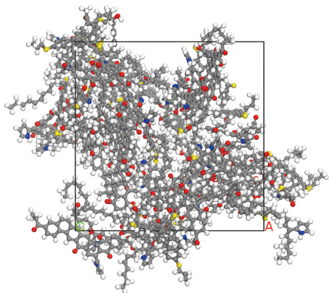
Fig. 2. A periodic box containing 10 kerogen molecules.
