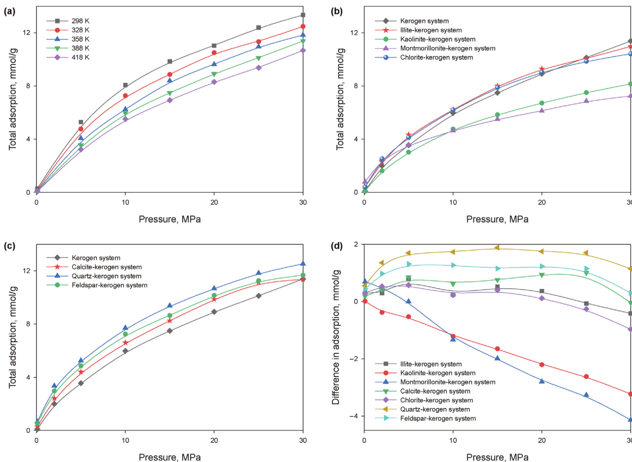
Fig. 10. Isothermal adsorption curves of methane in different systems. (a) Kerogen system; (b) clay-mineral composite model system; (c) non-clay mineral composite model system; (d) difference between the adsorption capacity of methane in different systems and the adsorption capacity of mono kerogen system.
