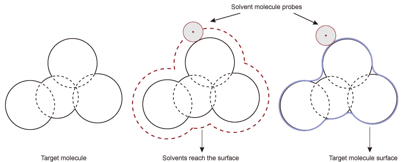
Fig. 16. Schematic diagram of Connolly molecular surface calculations (Revised according to (Yang et al., 2017)).
