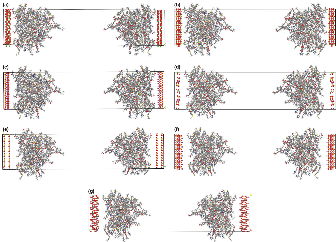
Fig. 8. Three-dimensional composite models of kerogen with inorganic minerals. (a) Calcite-kerogen composite model, (b) montmorillonite-kerogen composite model, (c) kaolinite-kerogen composite model, (d) chlorite-kerogen composite model, (e) quartz-kerogen composite model, (f) illite-kerogen composite model, (g) feldspar-kerogen composite model.
