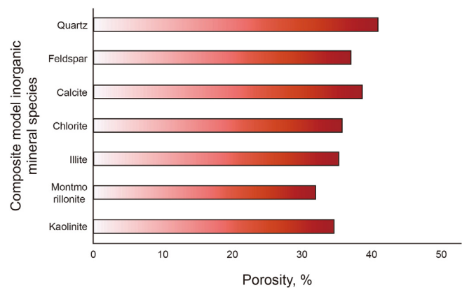
Fig. 17. Porosity of different shale composite systems.
