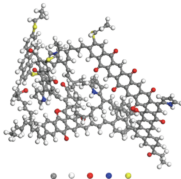
Fig. 1. Three-dimensional molecular structure of type II kerogen shale in the Longmaxi Formation in the Sichuan Basin (C 206 H 158 O 19 N 4 S 4 ) (The gray spheres represent carbon atoms, white spheres represent hydrogen atoms, red balls represent oxygen atoms, blue balls represent nitrogen atoms, and yellow balls represent sulfur atoms).
