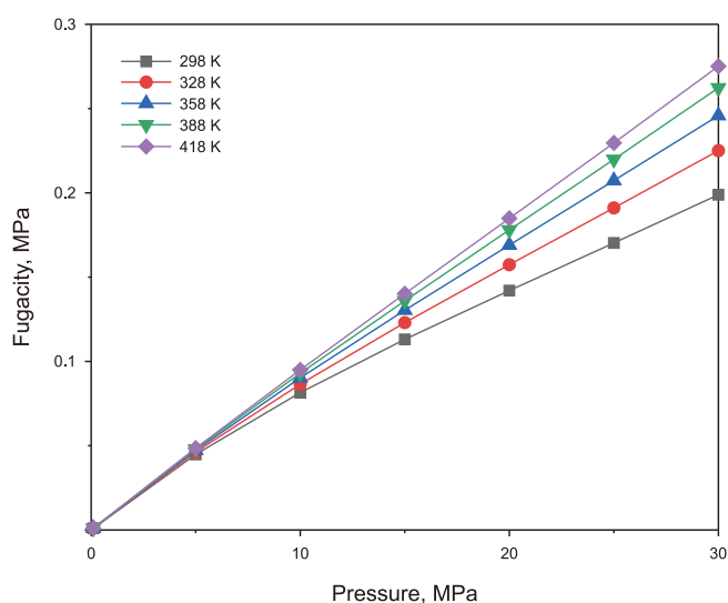
Fig. 9. The fugacity of methane at different temperatures as a function of pressure.
