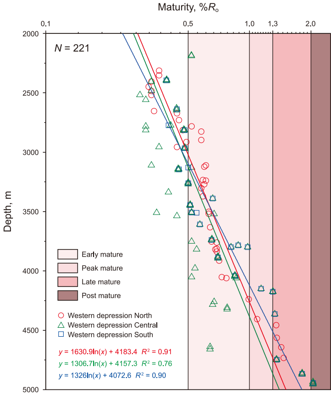
Fig. 13. Fitting study between R_o data and the corresponding depths in the Western Depression, with well S202 representing the northern side, wells SS3 and SG1 representing the central section, and well MS1 representing the southern side of the study area.
