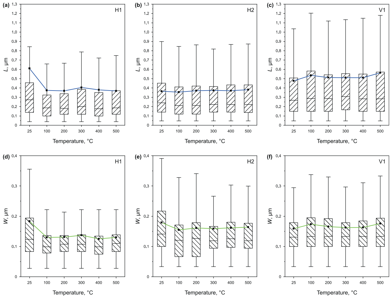
Fig. 6. Statistics of length ( L ) and width ( W ) recovered from machine learning. (a)–(c) L values for SEM images of the three samples; (d)–(f) W values for SEM captures.
