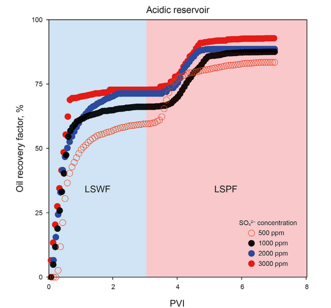
Fig. 13. The measured oil recovery by the injection water containing different \text{SO}_4^{2-} concentrations for acidic and neutral reservoir conditions.
