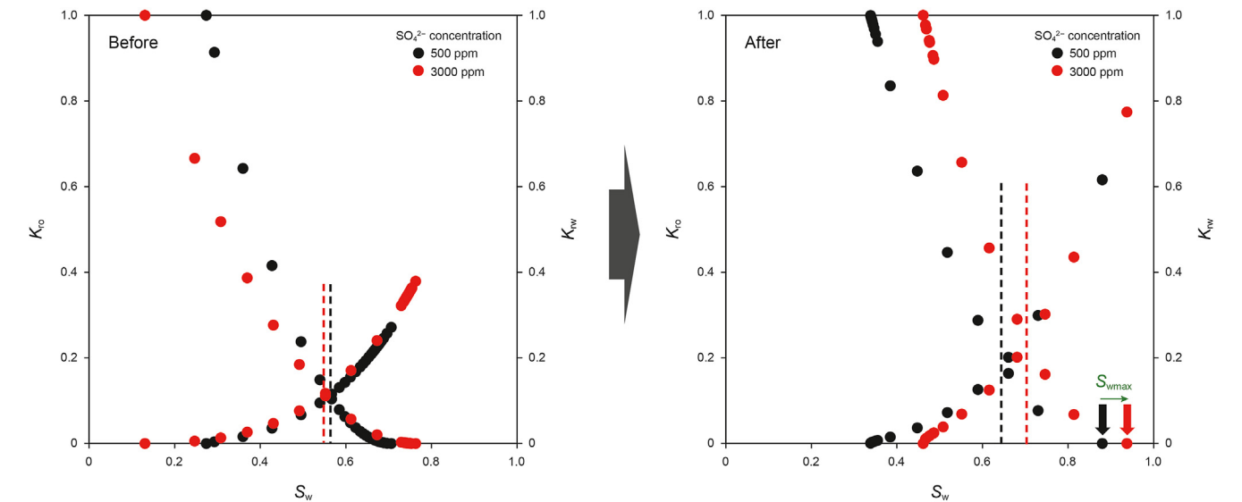
Fig. 12. The changes in relative permeability curves for the acidic reservoir condition.
