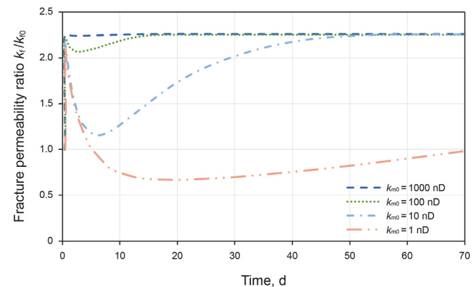
Fig. 8. Evolution of permeability for adsorbing gas (CO 2 ) under different initial matrix permeability values at a constant confining stress.
