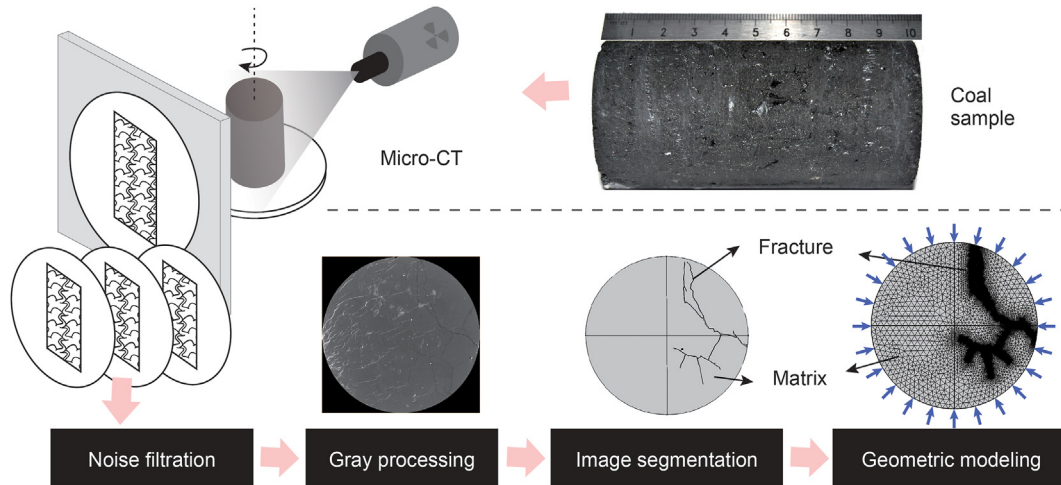
Fig. 2. Schematic diagram of CT data processing of the coal sample.
