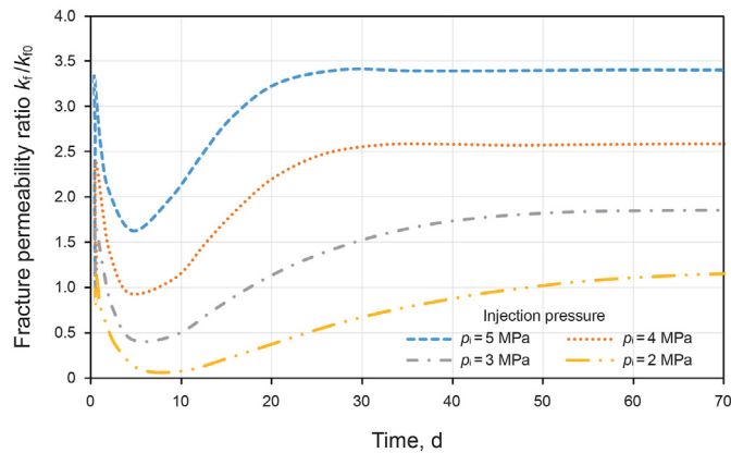
Fig. 6. Evolution of permeability for adsorbing gas (CO 2 ) under different injection pressures at a constant confining stress.
