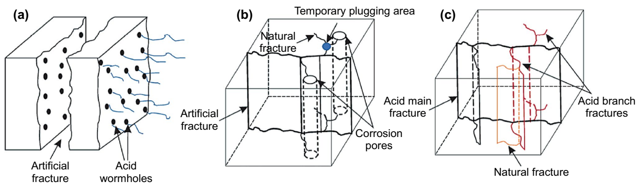
Fig. 4 Three-dimensional stimulation diagram of different types of reservoirs: a pore type, b fracture cavity type, c fracture type. Reprint permission obtained from Guo et al. (2020)
