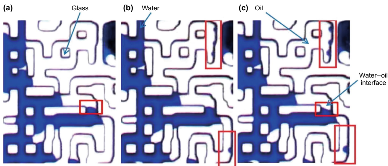
Fig. 7 Fluid distribution in a section of the micromodel (a) after WI and (b, c) after 19.6 and 47.12 h of CWI, respectively. Reprint permission obtained from Seyyedi et al. (2015)
