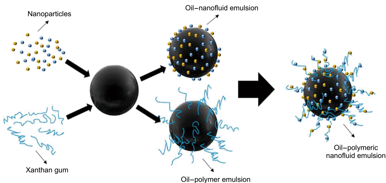
Fig. 12 Schematic diagram illustrating the trapped crude oil and low-salinity polymeric-nanofluid emulsion. Reprint permission obtained from Ali et al. (2019)
