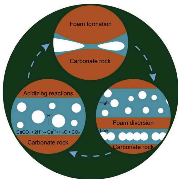
Fig. 3 Mechanism of in situ foam acidizing technology. Reprint permission obtained from Yan et al. (2019)
