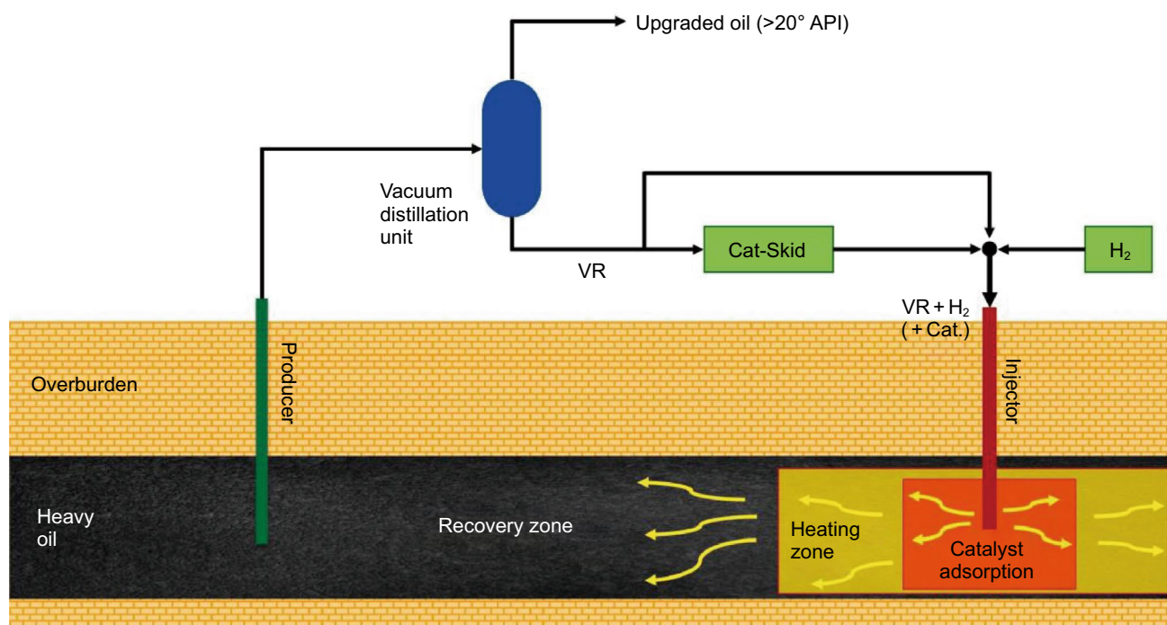
Fig. 14 Schematic of the ISUT for a carbonate reservoir. Reprint permission obtained from Elahi et al. (2019)
