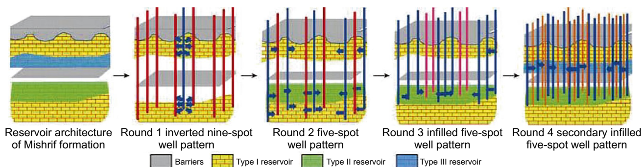
Fig. 8 Schematic diagram for different types of reservoirs developed by different well patterns. Reprint permission obtained from Song and Li (2018)
