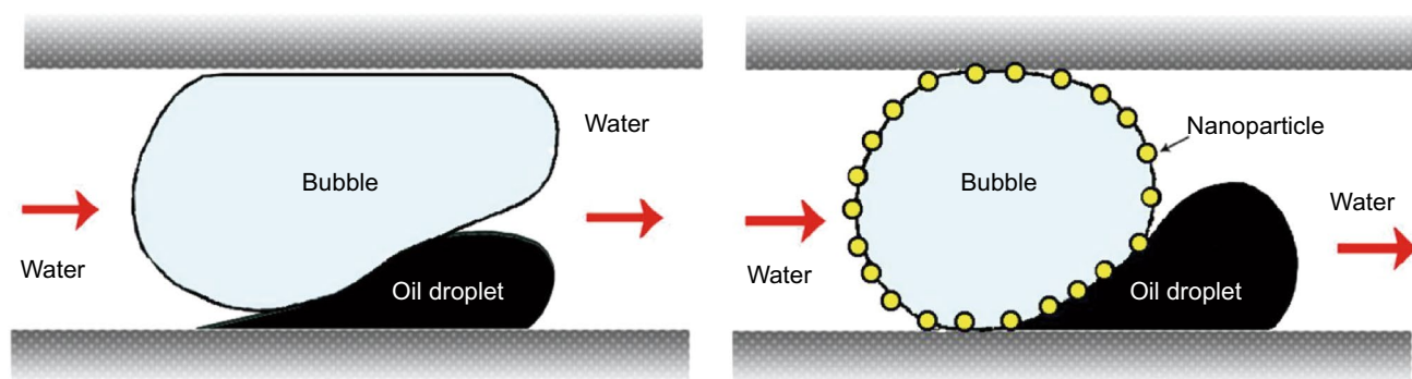
Fig. 13 Displacement differences for an oil droplet on a pore wall by SDS foam (left) and SiO 2 /SDS foam (right). Reprint permission obtained from Sun et al. (2014)
