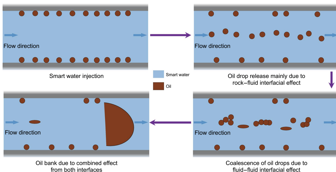
Fig. 6 Smart water flooding recovery mechanism using the combined effects from both fluid–fluid and rock–fluid interfaces. Adapted from Ayirala et al. (2016)
