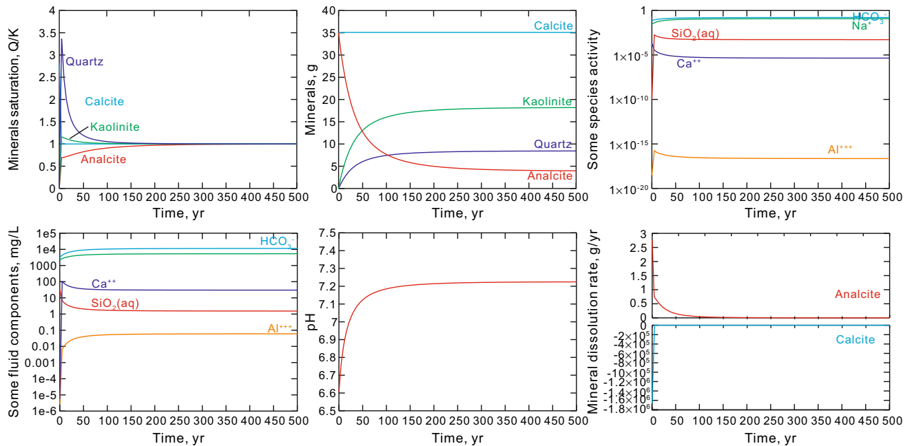
Fig. 13 Numerical simulation results of fluid-rock reactions in the calcite-analcite- \text{CO}_2 - \text{H}_2\text{O} system for extended periods of time (500 years)
