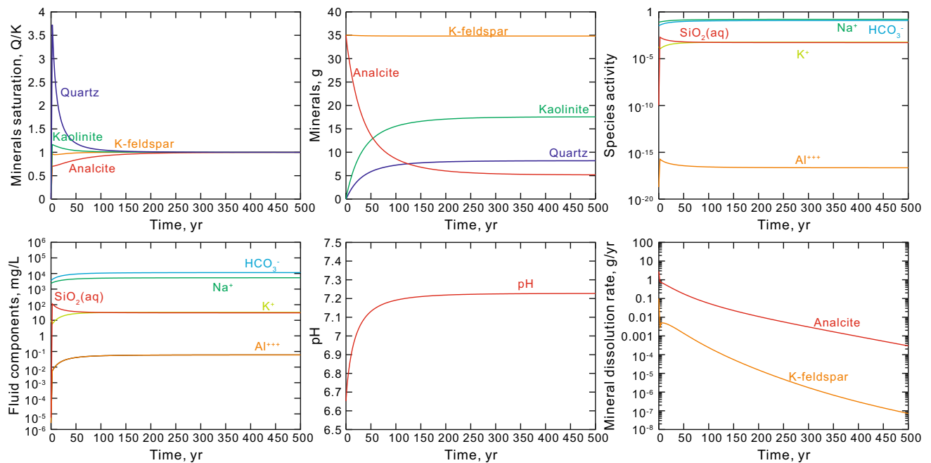
Fig. 14 Numerical simulation results of fluid-rock reactions in the analcite-K-feldspar- \text{CO}_2 - \text{H}_2\text{O} system for extended periods of time (500 years)
