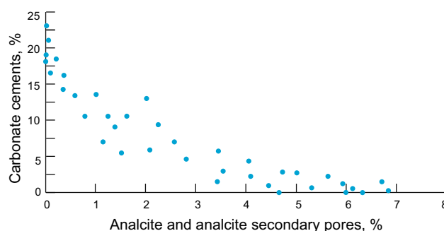
Fig. 5 Negative relationship between the amount of carbonate cement and the amount of analcite and analcite secondary pores in the reservoirs in the Xing'anling Group
